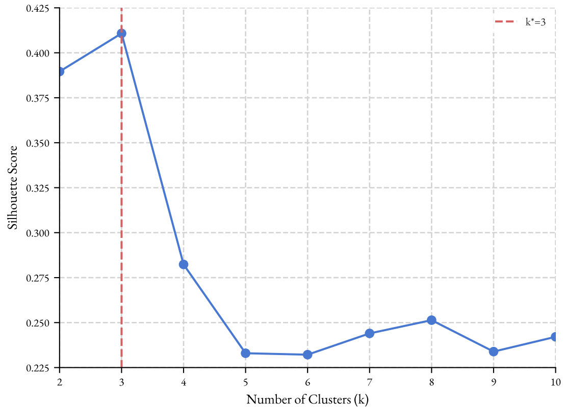
Silhouette Score for K-Medoids Clustering
