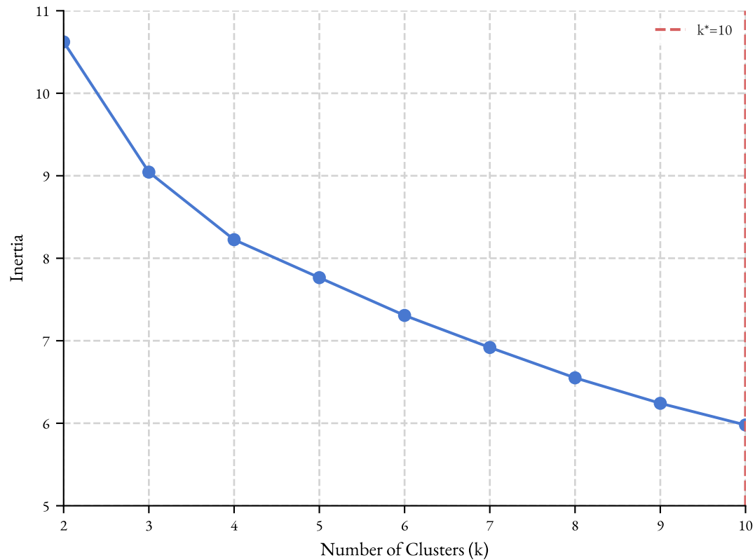
Elbow Method for K-Medoids Clustering
